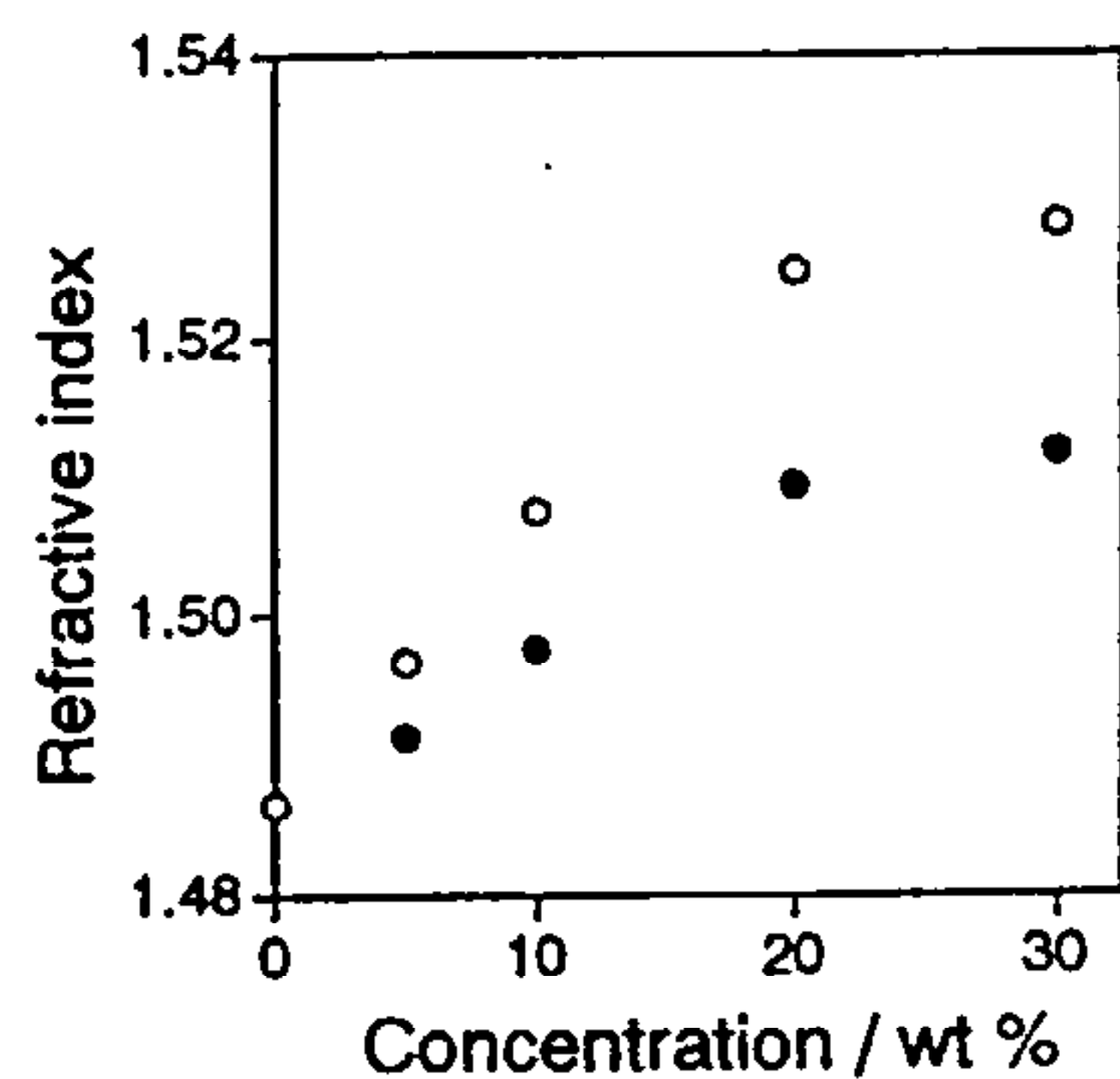
Figure 7. Refractive indices of PMMA films containing various weight fractions of \beta -AS before (open circle) and after 30 min of photoirradiation (filled circle).
