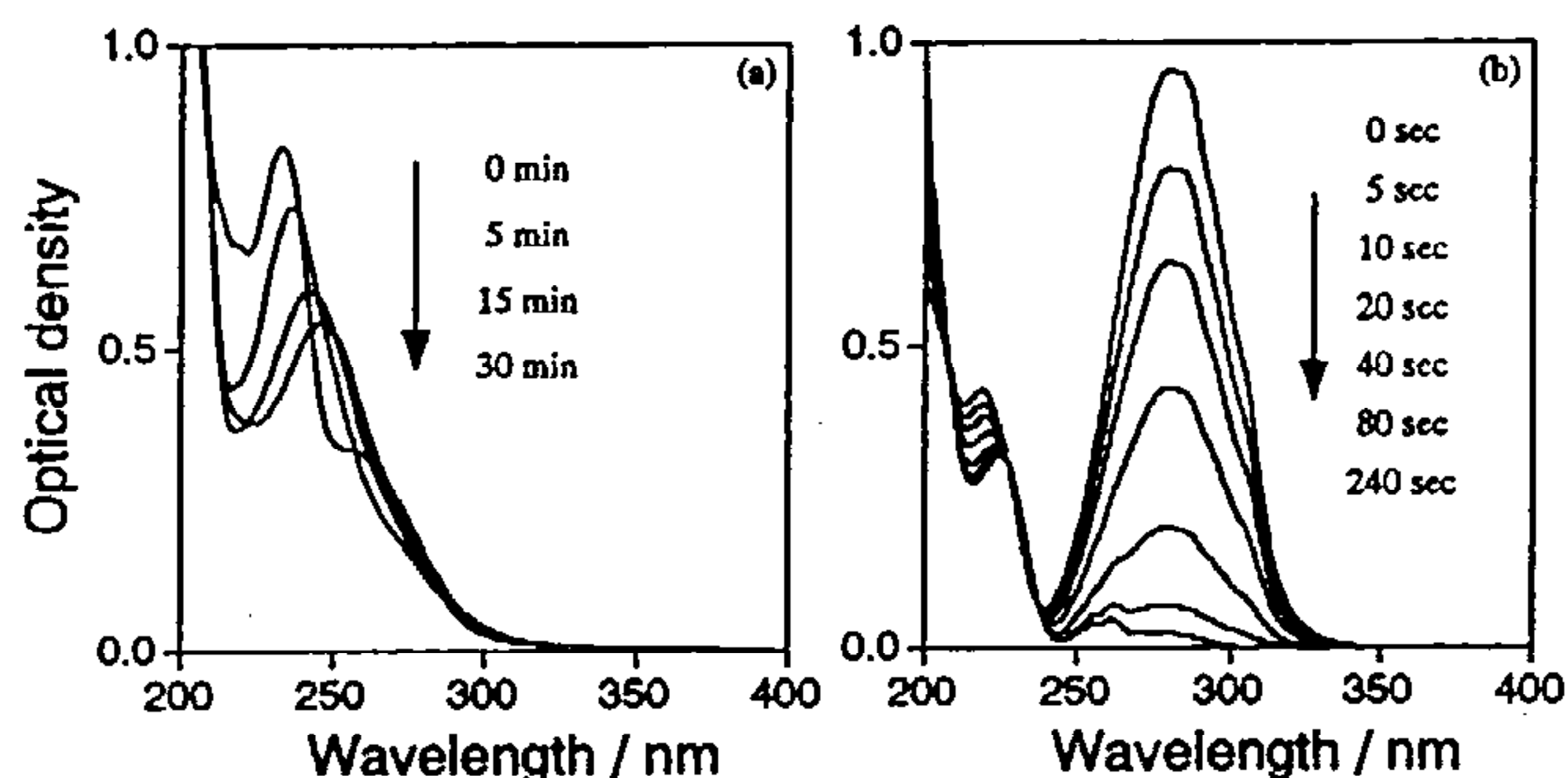
Figure 6. Absorption spectra of \alpha -AS and \beta -AS in acetonitrile solutions before and after photoirradiation. (a) \alpha -AS in 5.9 \times 10^{-5} \text{ mol/L} solution, (b) \beta -AS in 3.5 \times 10^{-5} \text{ mol/L} solution. Arrows show the direction of change during photoirradiation. Photoirradiation times are shown beside the arrows.
