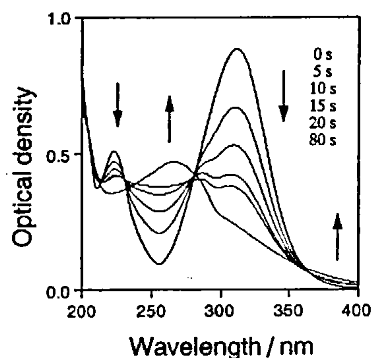
Figure 5. Absorption spectra of 4NAB in 5.0 \times 10^{-5} \text{ mol/L} acetonitrile solution before and after photoirradiation. Arrows show the direction of change during photoirradiation. Photoirradiation times are shown beside the arrow.
